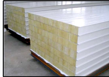
Sandwich Ceiling Panel
